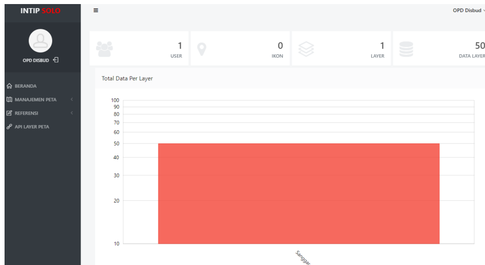
Gambar 2. Menu Dashboard
